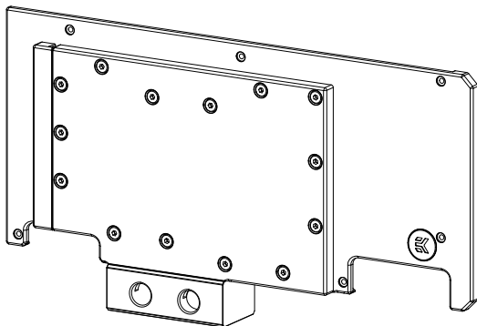
EK-Quantum Vector Strix RTX 3080/3080Ti/3090 Active Backplate
